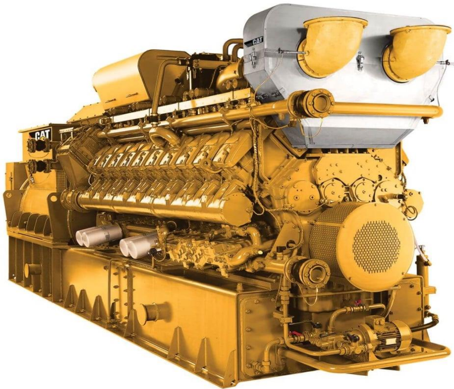
Figure 2: Caterpillar CG170-20 Twenty (20) Cylinder Engine Outline.
